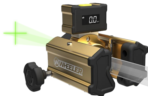
STEP 3 Bore Sight and Level Scope using Cross-beam Laser
